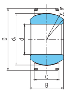
GEC(H)...XT
