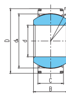
GEC(H)...XT-2RS
